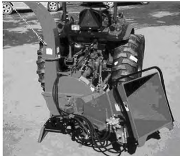
BX62/620R Hopper
