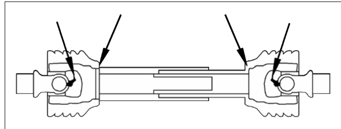
Fig. 38 PTO driveline
